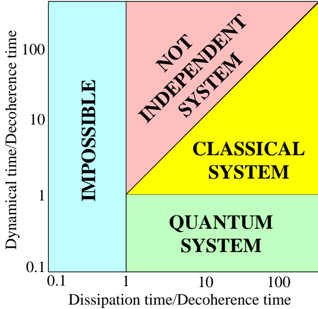
FIG. 1. The qualitative behavior of a subsystem depends on the timescales for dynamics, dissipation and decoherence. This classification is by necessity quite crude, so the boundaries should not be thought of as sharp.
